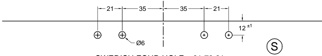
SWEDISH FOUR HOLE 21-70-21
