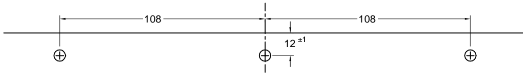
AMERICAN THREE HOLE 108-108
