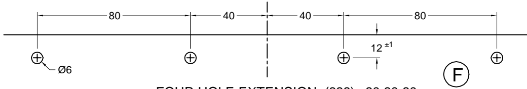
FOUR HOLE EXTENSION (888) 80-80-80
