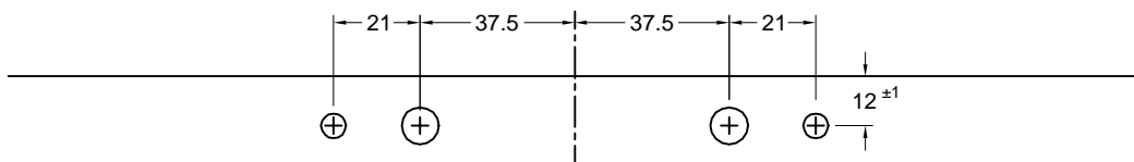
HOLE POSITION OF SPECIAL PUNCHING MACHINE
