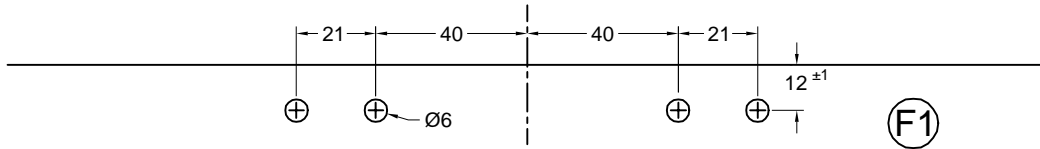
FOUR HOLE EXTENSION ISO 838 21-80-21
