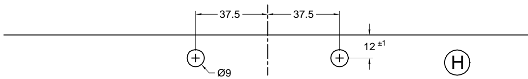
HYBRID TWO HOLE 80-70
